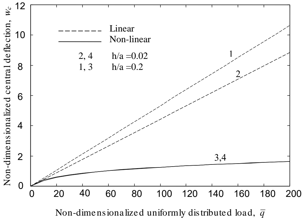
Fig. B.1 Variation of central deflection, \bar{w}_c with load, \bar{q} of thin ( h/a = 0.02 ) and thick ( h/a = 0.2 ) simply supported (SS5) square isotropic plate.
